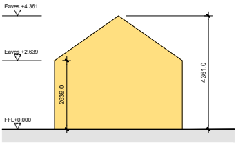
Existing Structure 2 - South Elevation Scale 1:200
