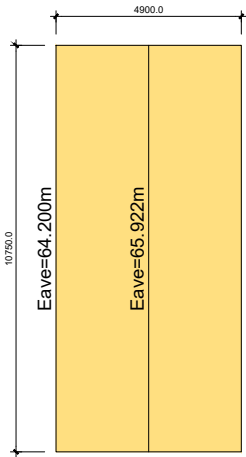
Existing Structure 2 - Plan Scale 1:200
