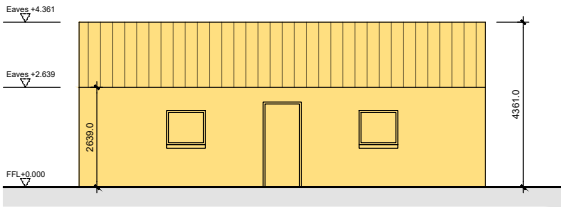
Existing Structure 2 - East Elevation Scale 1:200
