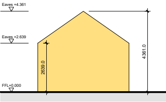
Existing Structure 2 - North Elevation Scale 1:200
