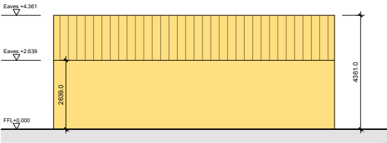
Existing Structure 2 - West Elevation Scale 1:200
